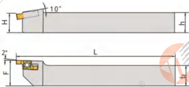
注意：左手刀具配GER系列刀片，右手刀具配GEL系列刀片 Note: Left tools match with right inserts; Right tools match with left inserts.
